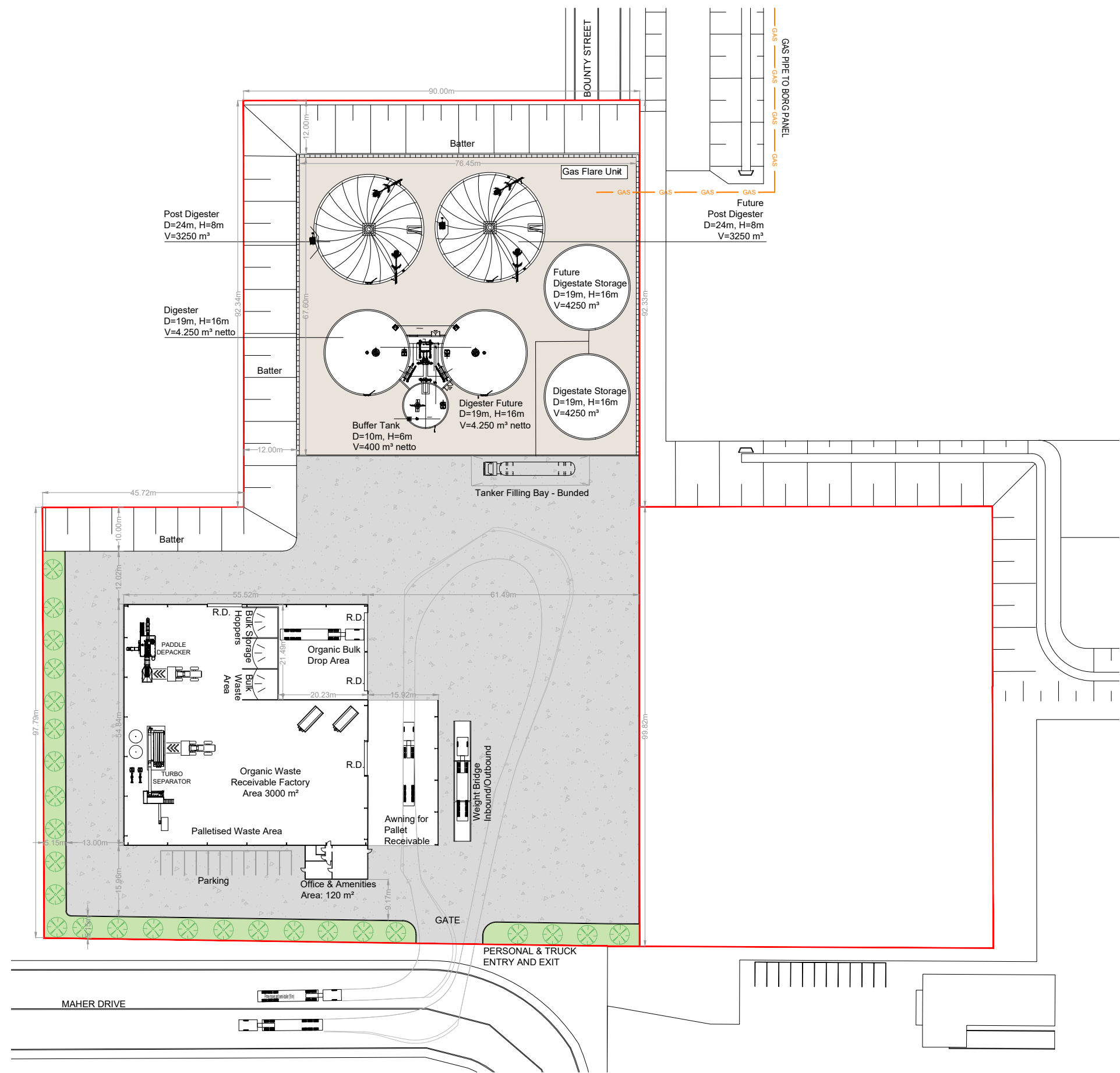
1 PROPOSED SITE PLAN SCALE: 1:500 @ A1
